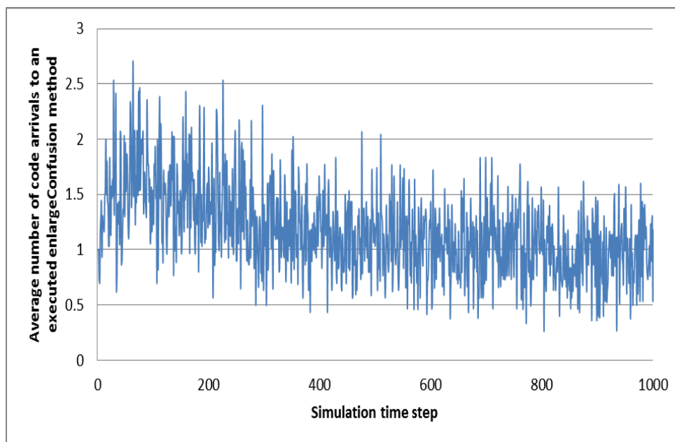
Fig. 5.2.1.8 Average number of code arrivals to an executed enlargeConfusion method: WM = 5; D = 5 (no chunking);
