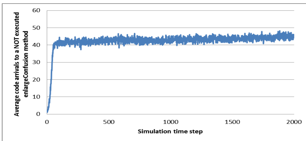
Fig. 5.2.1.7 Average number of code arrivals to a potential but NOT executed enlargeConfusion method: WM = 5; D = 5 (chunking);
