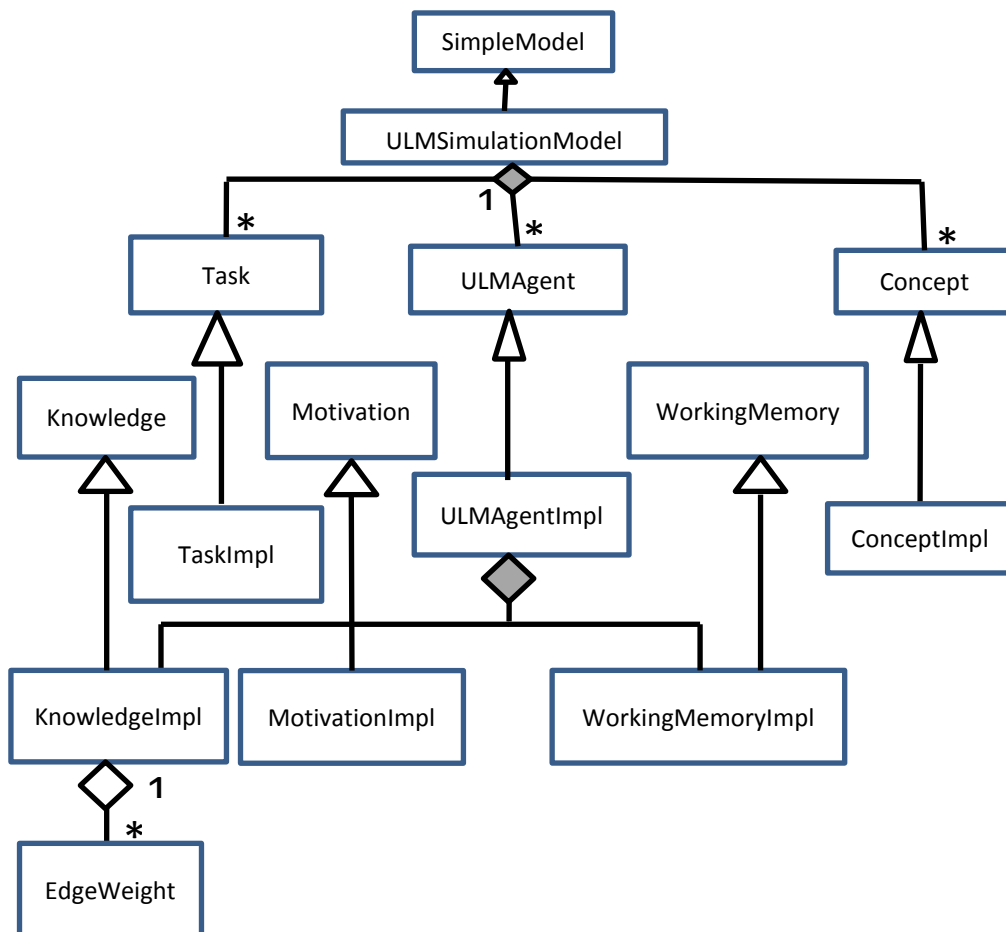
Figure 4.1 UML Class Diagram
